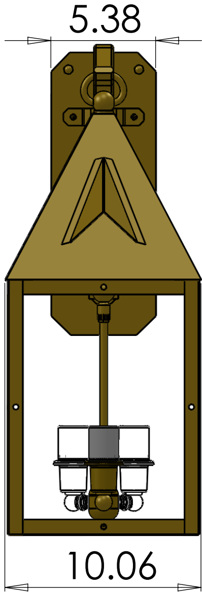
Front View
